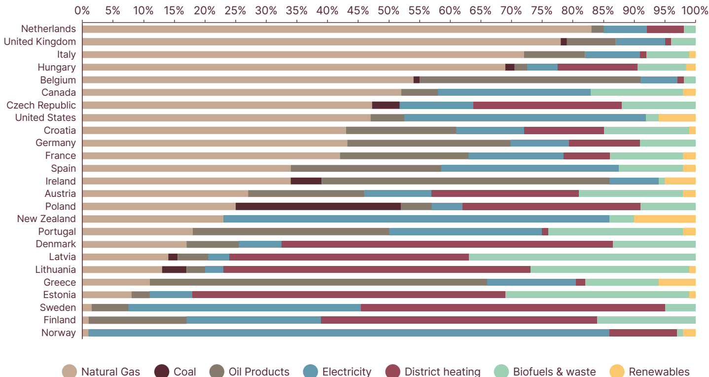
Fuel share (%) for residential and commercial heating demand in selected OECD countries, 2014 % of total
