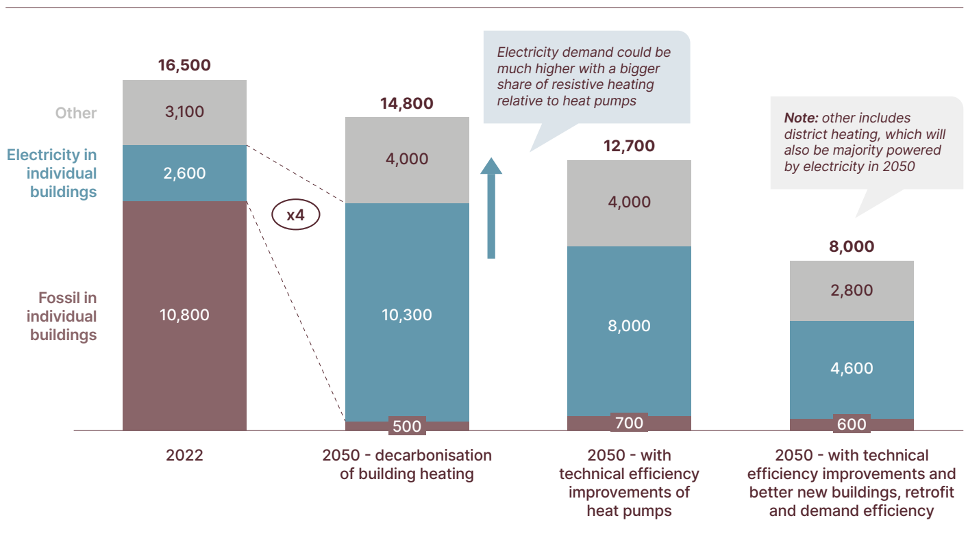
Global final energy demand for heating by fuel in 2050 TWh
