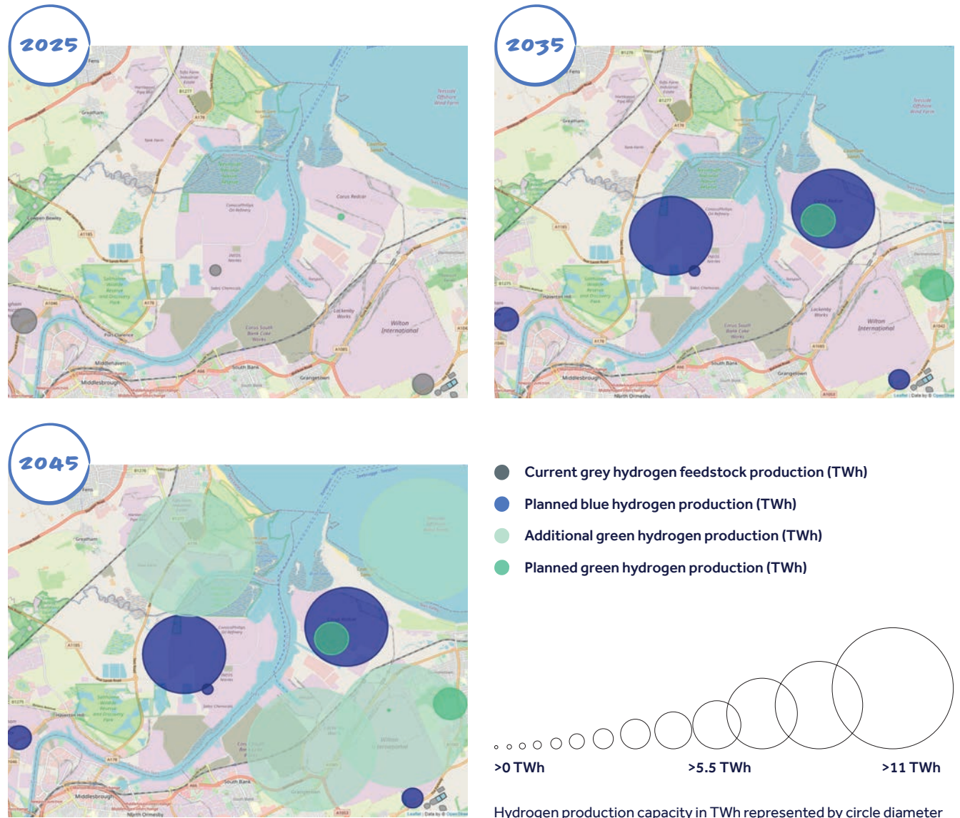
Hydrogen production capacity in TWh represented by circle diameter
