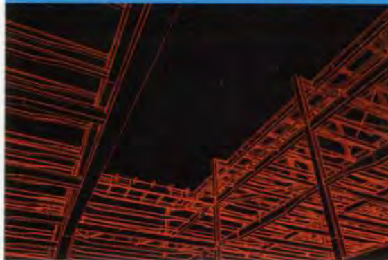
6. Extract from XSTEEL 3D computer model of the atrium structure, without atrium roof details.
