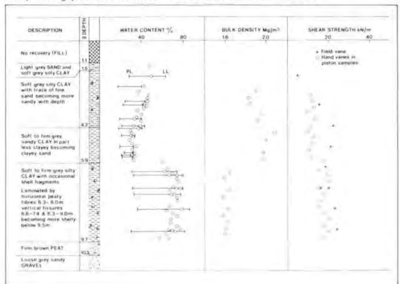
Fig. 4 Borehole profile
