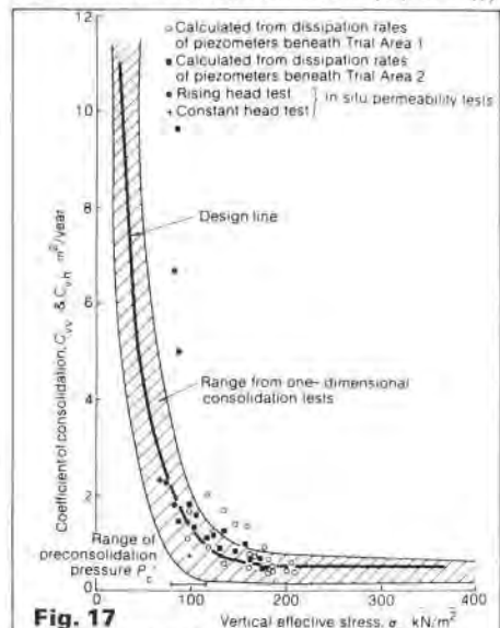
Fig. 17 Variation of coefficient of consolidation with vertical effective stress
