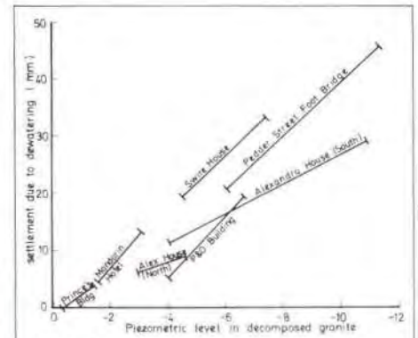
Fig. 23 Initial measurements of settlements of high rise piled building due to dewatering (prior to main excavation)
