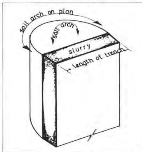
Fig. 10 Model of soil arching for preliminary assessment of earth pressures around slurry trench
