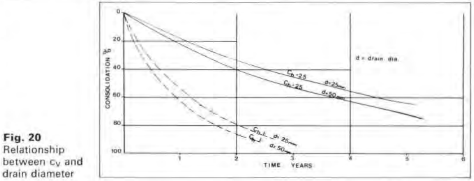
Fig. 20 Relationship between C_v and drain diameter
